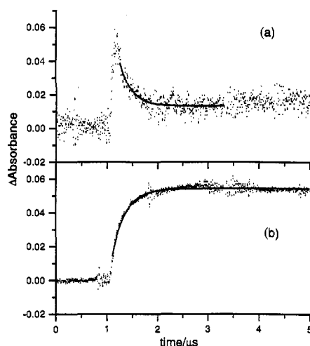
Figure 3. Kinetic traces of the IR absorbance of \text{Re}(\text{Bz})(\text{CO})_3(\text{iPr-DAB}) in n -heptane measured after 532 nm, 10 ns excitation: (a) immediate formation and subsequent decay of the primary intermediate monitored at 2014.9 \text{ cm}^{-1} , \tau = 210 \text{ ns} ; (b) photoproduct formation ( \tau = 260 \text{ ns} ) monitored at 1898 \text{ cm}^{-1} .
