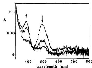
Figure 1. Time-resolved UV-vis spectra of \text{Re}(\text{Bz})(\text{CO})_3(\text{iPr-DAB}) in toluene measured at 30, 230, and 430 ns after the excitation. Spectra are corrected for the bleached ground state absorption.
