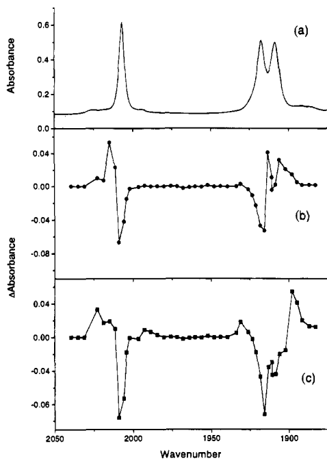
Figure 2. (a) FTIR spectrum of \text{Re}(\text{Bz})(\text{CO})_3(\text{iPr-DAB}) in n -heptane. (b) Difference time-resolved IR spectrum measured 100 ns after excitation. (c) Difference time-resolved IR spectrum measured 3.5 \mu\text{s} after excitation. Sample concentration 5 \times 10^{-4} M, optical path length = 2 mm.
